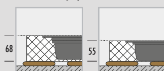
TUB-COMBI(-S) MQ SET 300
