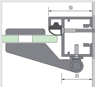
frame profile door hinge, wall connection
