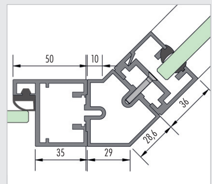
frame profile with corner profile 135° + wall profile
