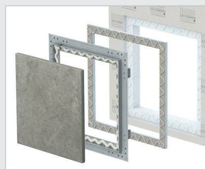
Application with natural stone: without front panel / fillers under frame
