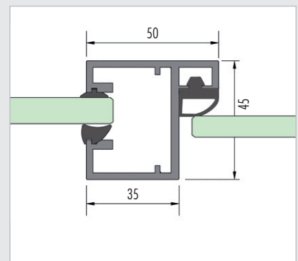
frame profile, connection wall profile
