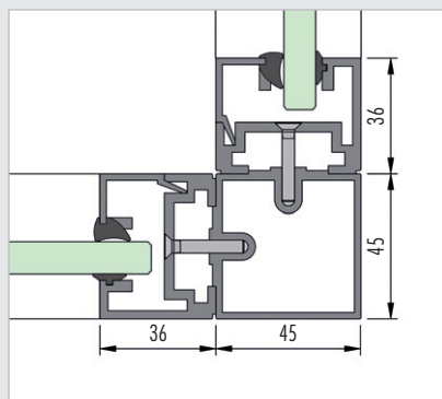
2x wall profile with corner profile 90°
