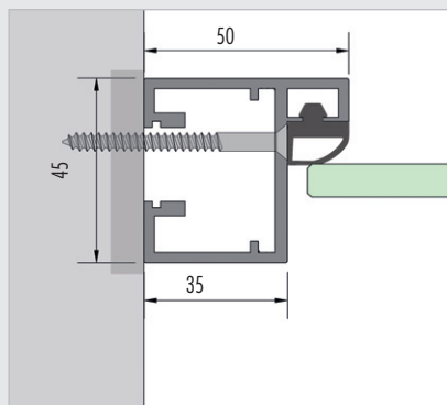
frame profile, wall connection
