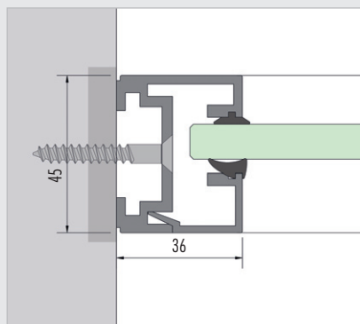
wall profile, wall connection
