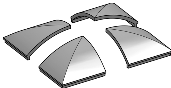
Cross-vault roof shape – CONCEPT-DA-CROSS
