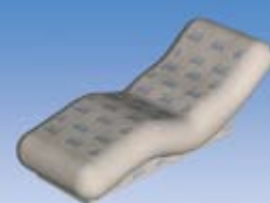
RELAX-RL-BELUGA
