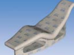
RELAX-RL-FIGURA
