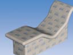
RELAX-RL-DREAM
