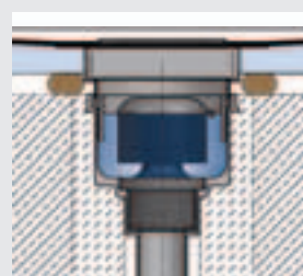
■ TUB-BAS-S FIRE STOP
